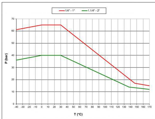
Pressure-temperature chart
